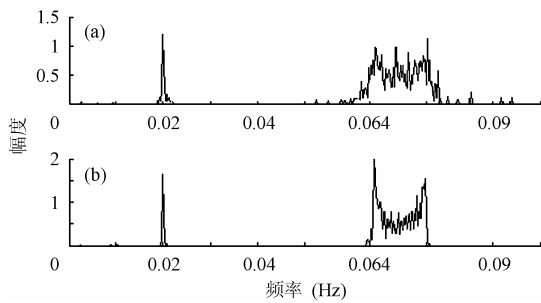
图 7 混合信号的边际谱 (a)基于 Hilbert 变换算法 (b)基于过零点-极点估计算法 Fig.7 Mixture signal's marginal spectrum (a) Algorithm based on Hilbert transform (b) Algorithm based on zero-crossing and extremum estimation algorithm
